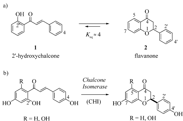
Figure 1. Cyclization of 2'-hydroxychalcones to flavanones. a) Most simple model reaction. b) Flavonoid biosynthesis.
