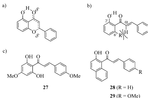
Figure 6. a) Hydrogen-bonding stabilization of the chalcone cyclization transition-state. b) Destabilizing effects of a 6'-substitution. c) Examples of ground-state destabilized chalcones used in this study.
