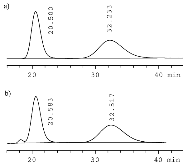
Figure 5. HPLC traces of 23 . a) Racemic reference. HPLC: Chiralcel-OJ , EtOH/ n -heptane, 1:1 (v/v), 0.7 mL/min, \lambda = 280 nm, \alpha = 1.707 , R_S = 2.265 ; integrals 50.1% and 49.9%. b) Product from the CSA-catalyzed cyclization of 24 ; impurity at t_R = 19 min; integrals 49.9% and 48.7%.
