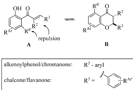
Figure 7. Structural factors in cyclization equilibria leading to chromanones/flavanones.
