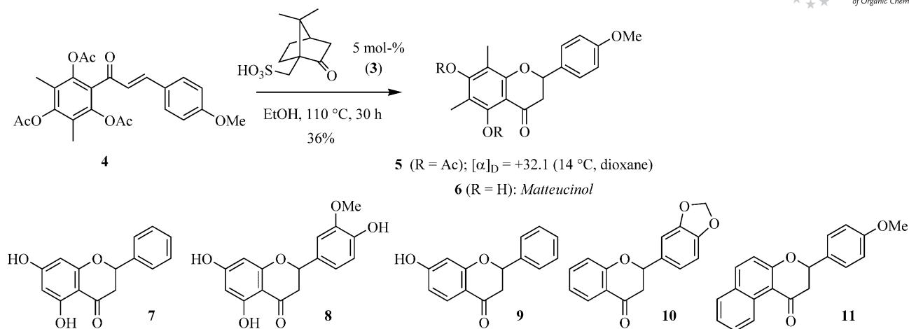
Figure 2. Experiments of Fujise et al. concerning the asymmetric cyclization of chalcones to flavanones. Chalcone precursors of 7 and 8 were the respective chalcone triacetates.
