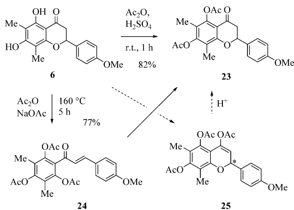
Scheme 3. Derivatization of matteucinol.
