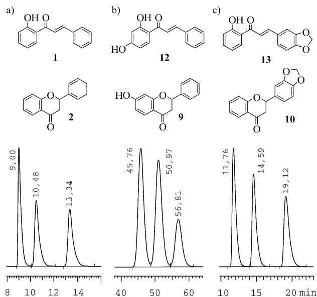
Figure 4. HPLC traces of reaction mixtures from CSA-catalyzed cyclizations of 2'-hydroxychalcones to flavanones. a) Cyclization of 1 to 2 . Chiralcel OD , n -heptane/ i PrOH, 97:3, 1 mL/min, \lambda = 254 nm. Peaks for 1 (integral 36.29%), 2 (integral 31.86%), ent - 2 (integral 31.85%). b) Cyclization of 12 to 9 . Chiralcel OJ , n -heptane/EtOH, 95:5, 1.2 mL/min, \lambda = 277 nm; peaks for 9 (integral 40.24%), ent - 9 (integral 40.62%), 12 (integral 19.13%). c) Cyclization of 13 to 10 . Chiralcel OD , n -heptane/ i PrOH = 95:5, 1 mL/min, \lambda = 254 nm, peaks for 13 (integral 36.03%), 10 (integral 31.93%), ent - 10 (integral 32.04%).
