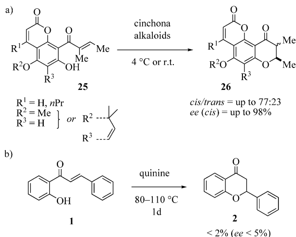
Scheme 4. Cinchona catalysis of alkenoyl-phenol cyclization. a) Results of Ishikawa and co-workers. [30] b) Unsuccessful extension to 2'-hydroxychalcone.
