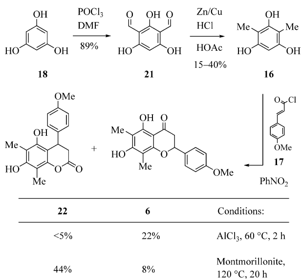
Scheme 2. Synthesis of matteucinol.
