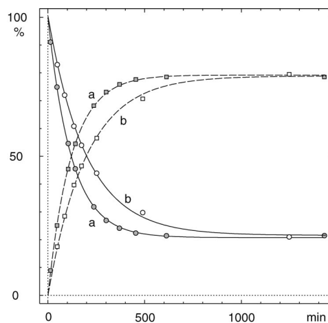
Figure 3. Reaction progress curves for cyclization of 1 to 2 in n BuOH at 120 °C. Solid lines: amount of 1 (%), dashed lines: conversion to 2 (%). a) Filled symbols: reaction in the presence of 20 mol-% of CSA. b) Open symbols: reaction without added catalyst (background reaction).
